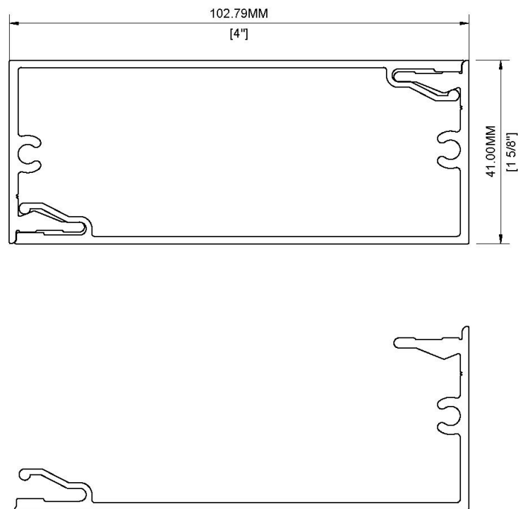
FIGURE 3—LINK & LOCK BATTENS (4-INCH PIECE TUBE AS SHOWN, ALSO AVAILABLE IN 2, 6 AND 8-INCH TUBES)
